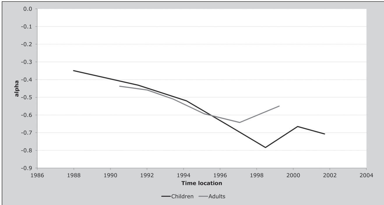
FIGURE 33.3 Alpha plot, after fitting \beta iteratively, Dominican Republic
